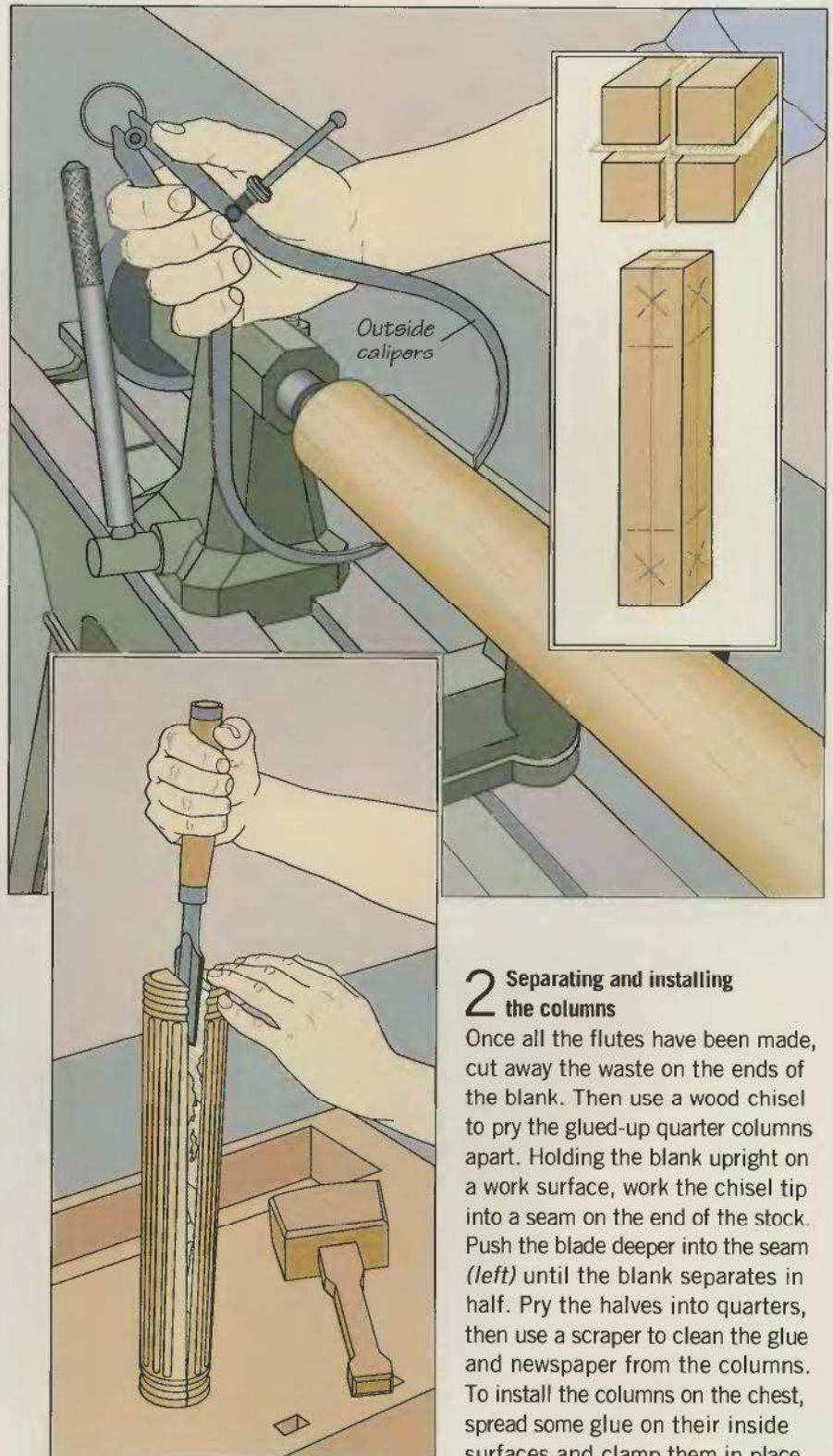
Fluted quarter columns add a strong visual framework to the highboy.
